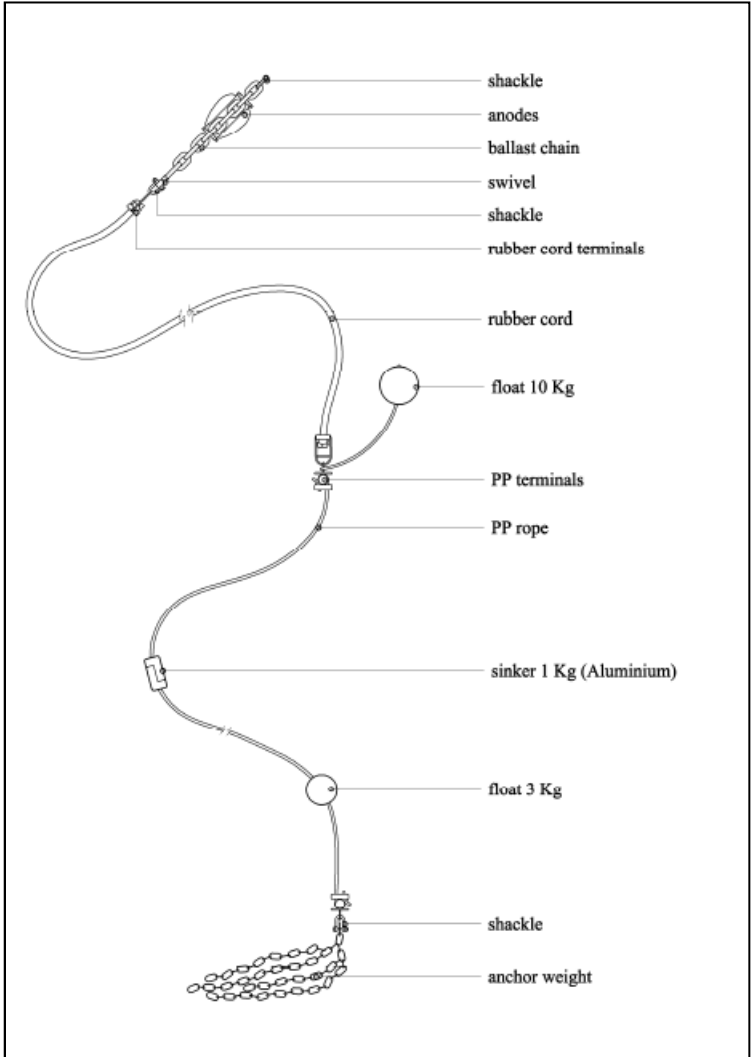
Figure 2: Directional Wave Rider and Mooring System
