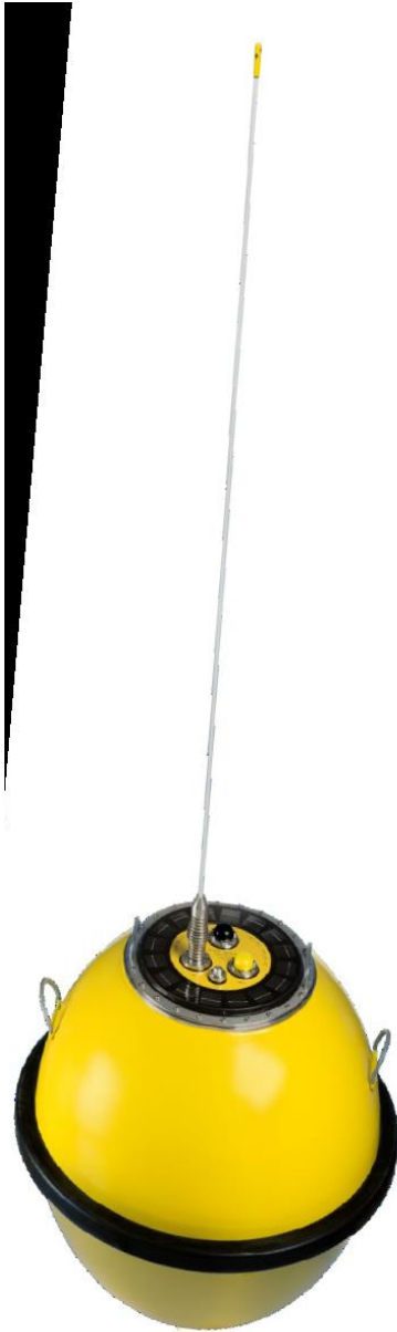
Figure 2: Directional Wave Rider and Mooring System
